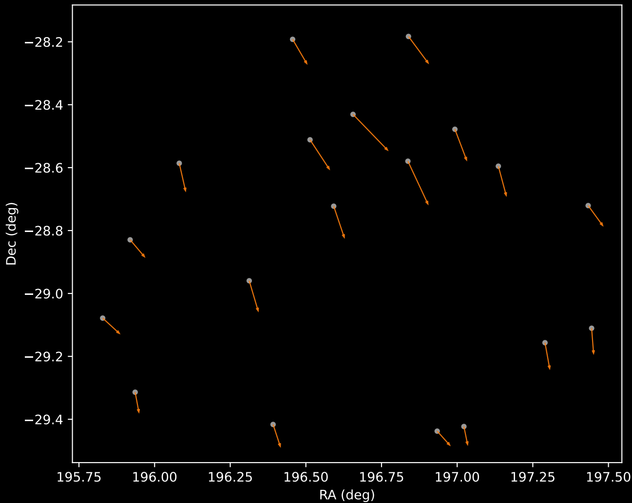
GALAH DR4 Cluster 2 Proper Motion Vectors (n=19)
