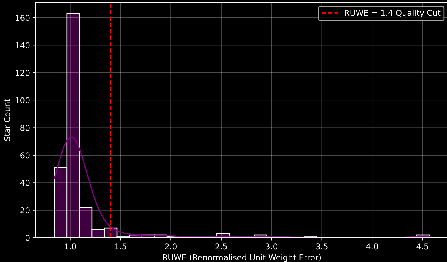
GALAH DR4 Field [2547] RUWE Distribution (n= 268)
