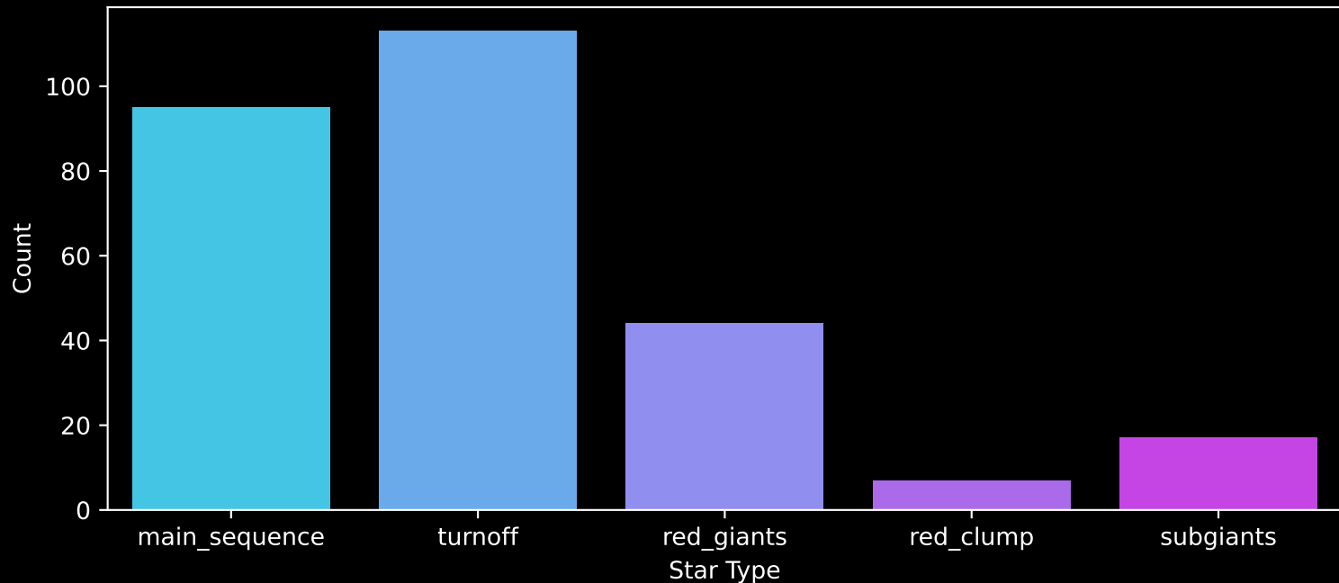
GALAH DR4 Field: [2547] Count plot of Star Type
