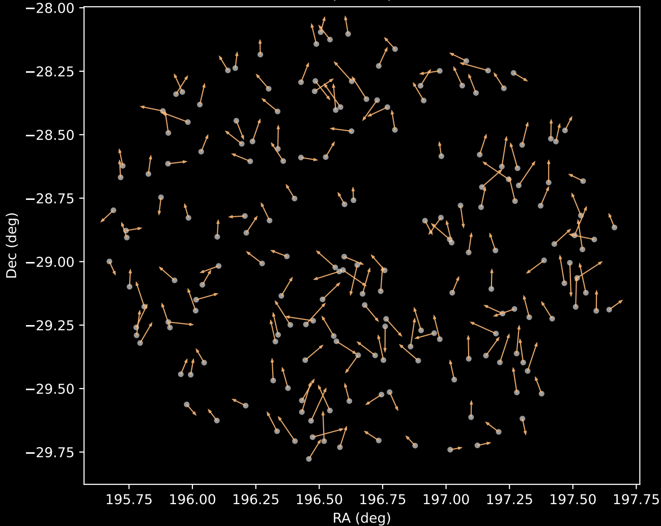
GALAH DR4 Cluster 3 Proper Motion Vectors (n=187)
