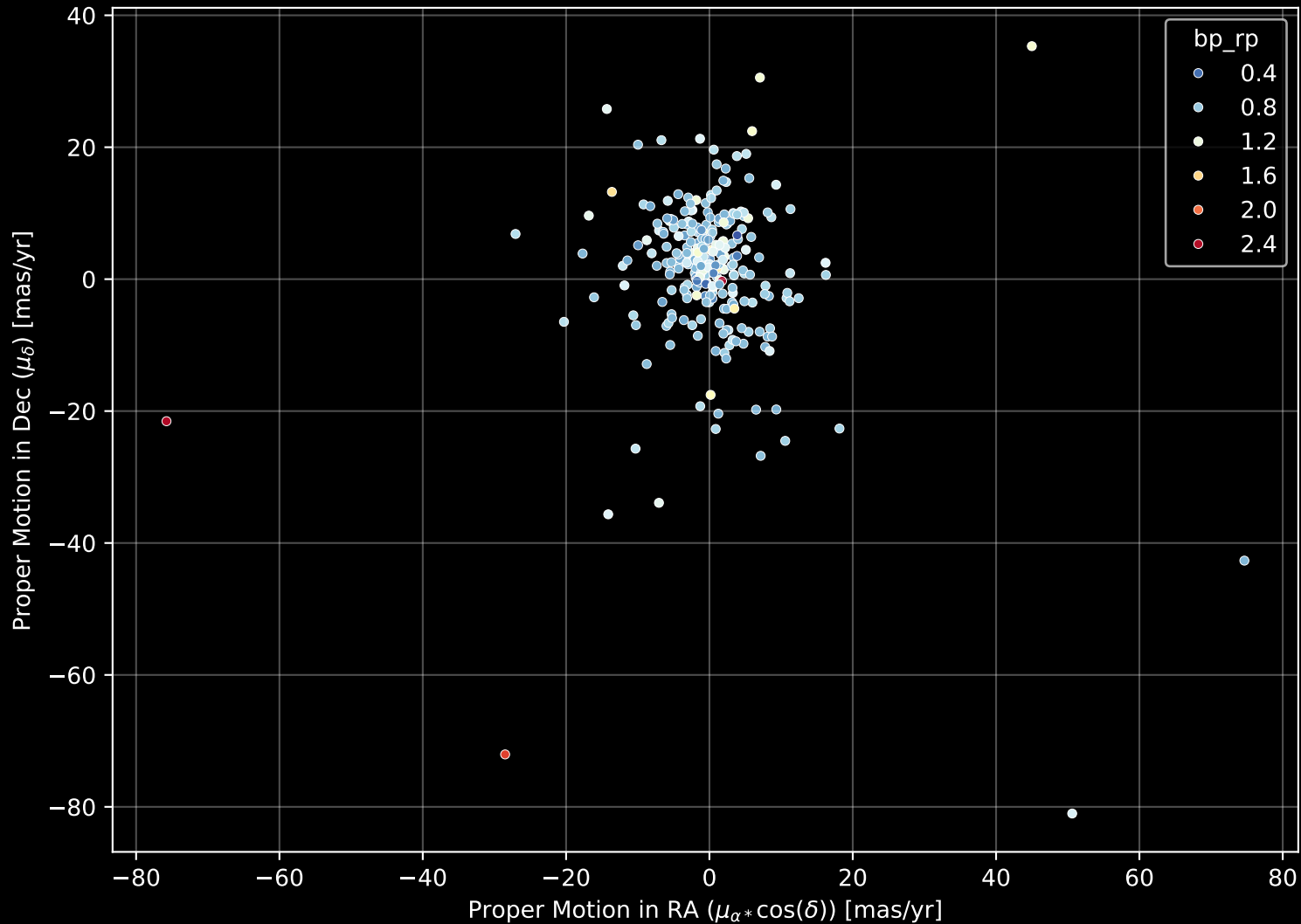
GALAH DR4 Field: [2547] Proper Motion Diagram (n= 276)
